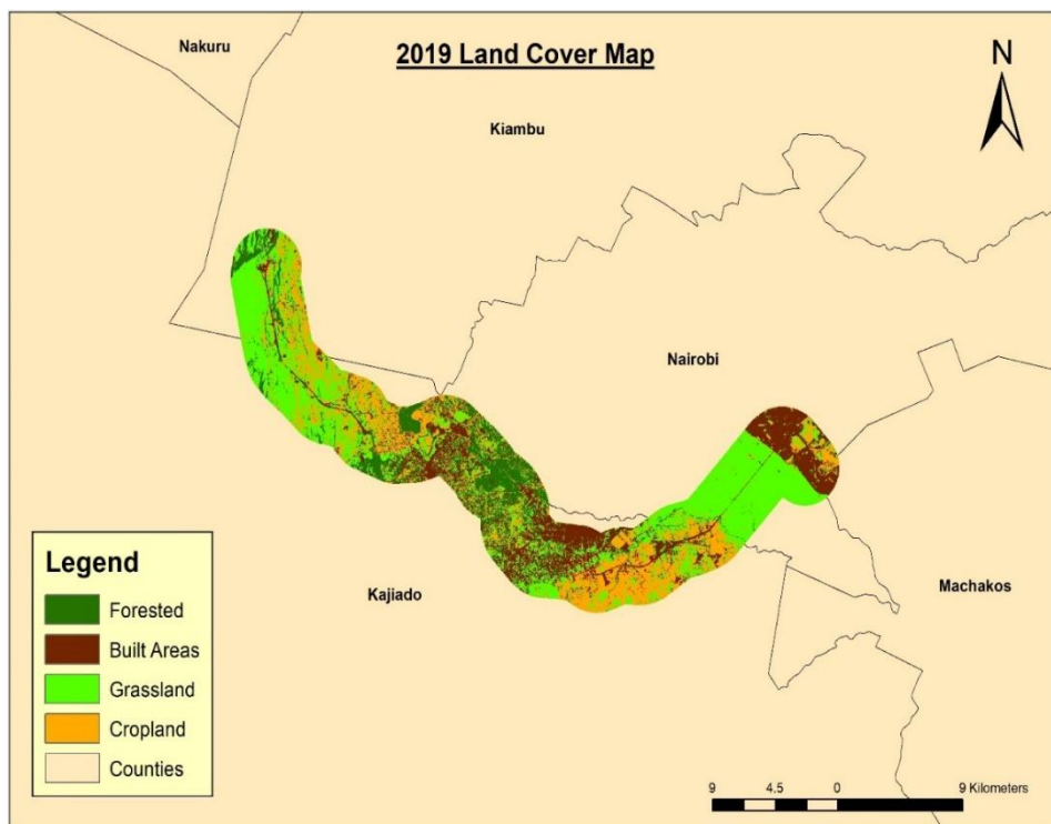
Fig. 3. Land cover change classification results for 2019
