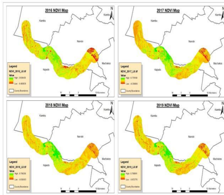
Fig. 6. Normalized Difference Vegetation Index maps for 2016 to 2019
