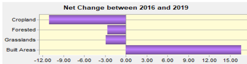
Fig. 5. Net land cover changes between 2016 and 2019 (in sq. km)
