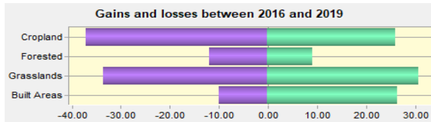
Fig. 4. Land cover classes gains and losses between 2016 and 2019
