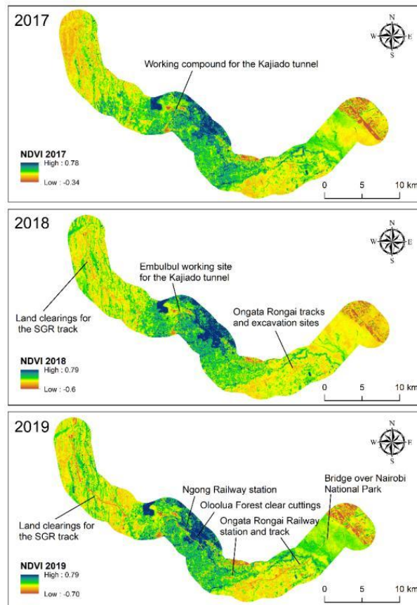
Fig. 7. NDVI based land cover change for 2016 to 2019
