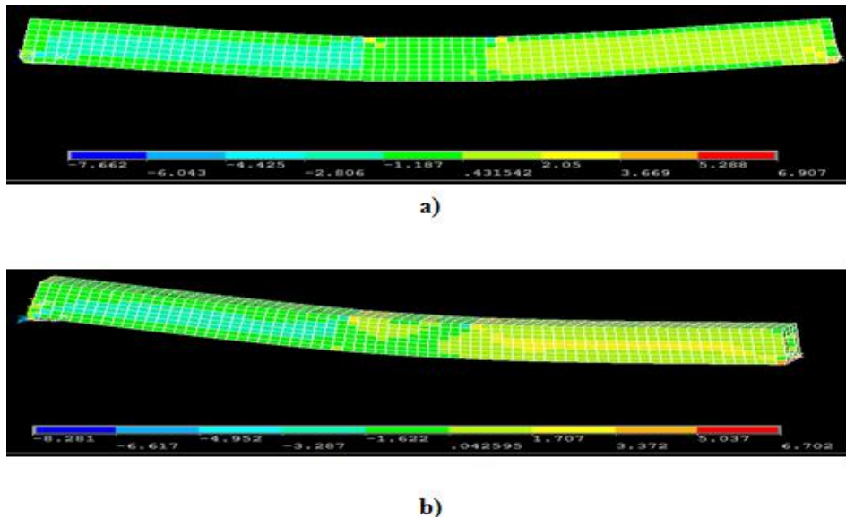
Fig. 12. NLFEA shear stresses a) Shear stresses for BOX1; b) Sample of shear stresses for different specimens
