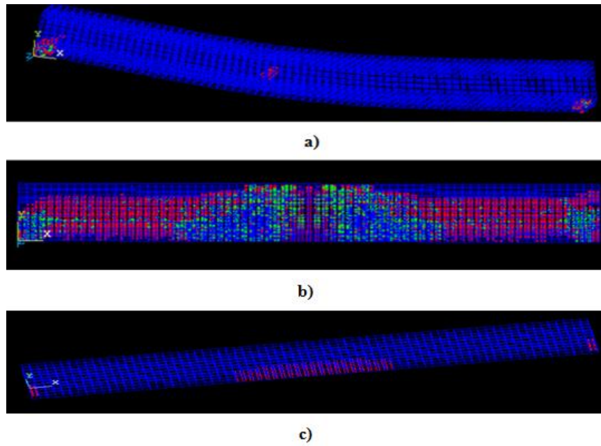
Fig. 9. Sample of crack pattern for control specimen a) first cracks; b) cracks at failure; c) sample of cracks for specimens in group 1 and 2
