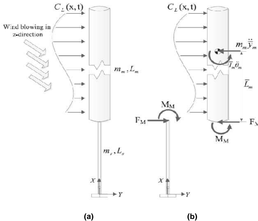
Fig.10(a) Schematic model of BWT (b) Free body diagram (chizfahm et al. 2008)
