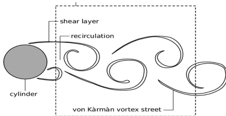
Fig. 2. Configuration of the cylinder wake Gerrard (1966) [9]
