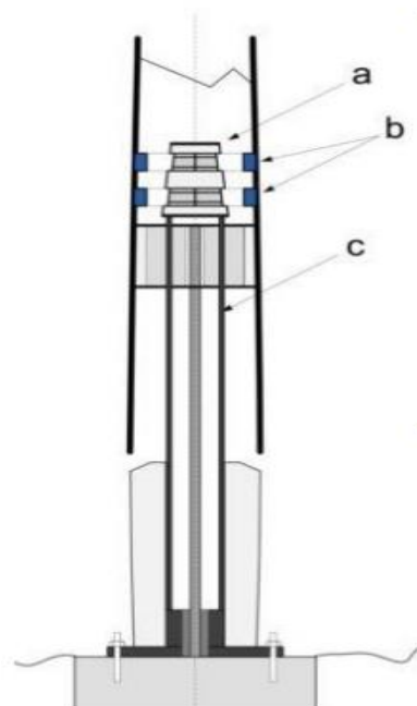
Fig. 9. Arrangement of alternator and tuning system (a) stator (b) permanent magnets and (c) structure (Vortex Bladeless S.L., 2018)
