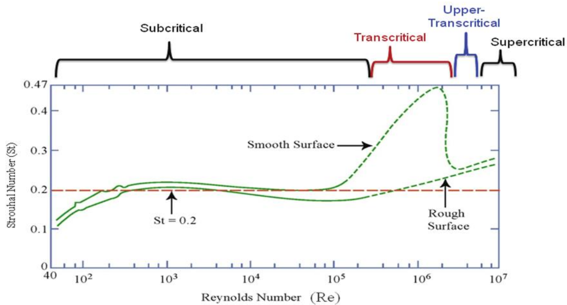
Fig. 5. Relationship between Strouhal number and Reynolds number for circular cylinders. (Roshko 1954)
