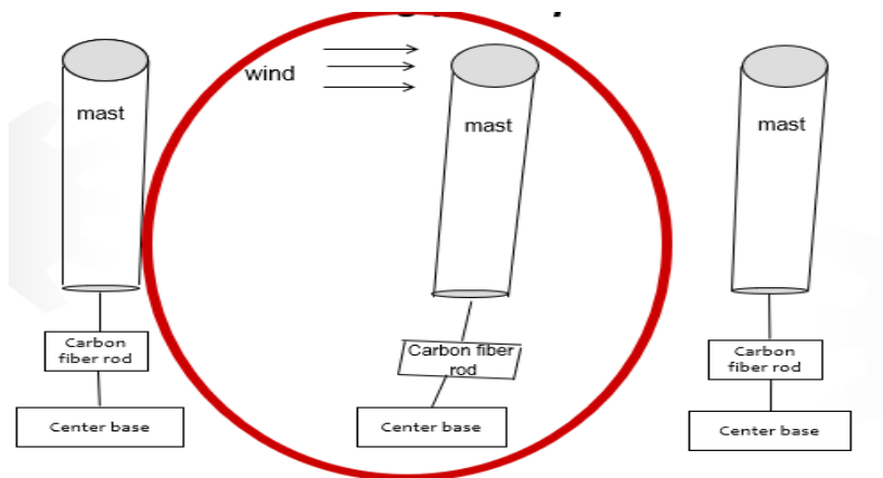
Fig. 8. Schematic diagram of BWT Working principle (Vortex Bladeless S.L., 2018) [18]
