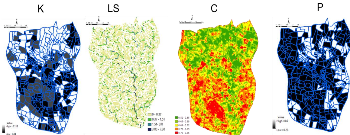
Fig. 3 B. The maps of K, LS, C, P of the RUSLE for soil loss estimation
