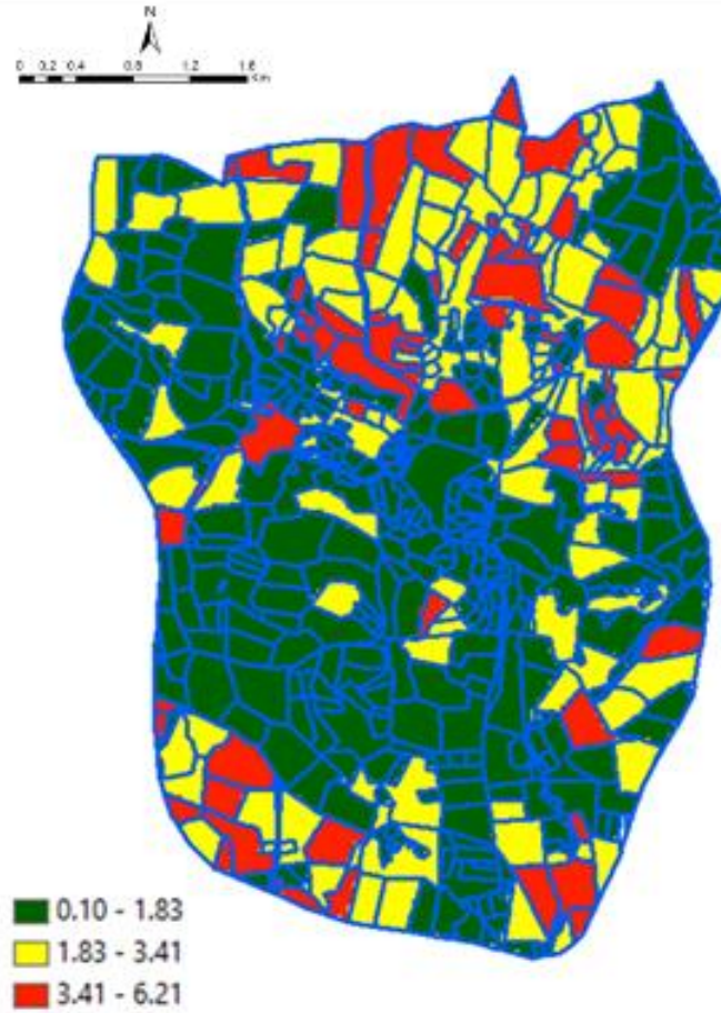
Fig. 4. Soil erosion (t /ha/Year) estimation using Revised Universal Soil Loss Equation (RUSLE)
