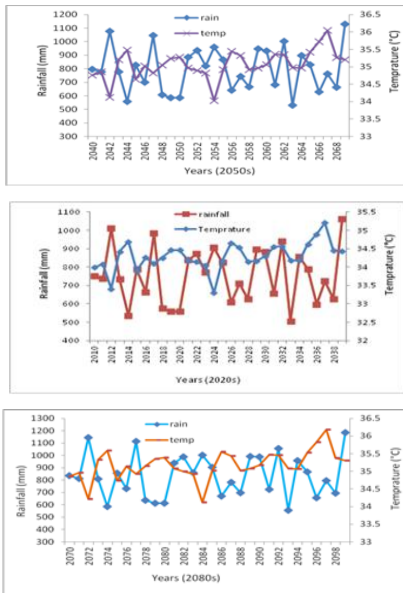
Fig. 2. The 2020s, 2050s and 2080s Rainfall and temperature graph
