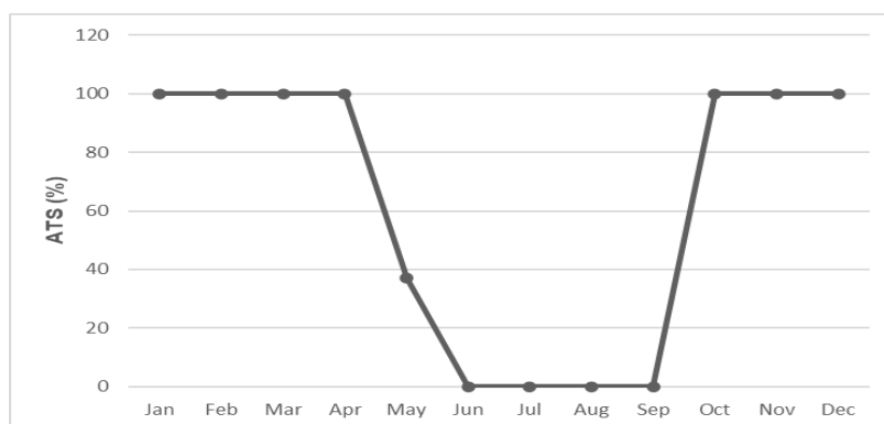
Fig. 4. Groundwater Availability in Mundri
