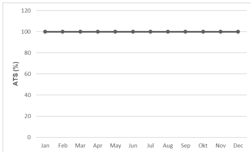
Fig. 5. Groundwater Availability in Bogorejo
