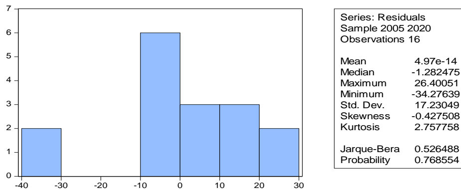
Fig. 1. Normality tests
