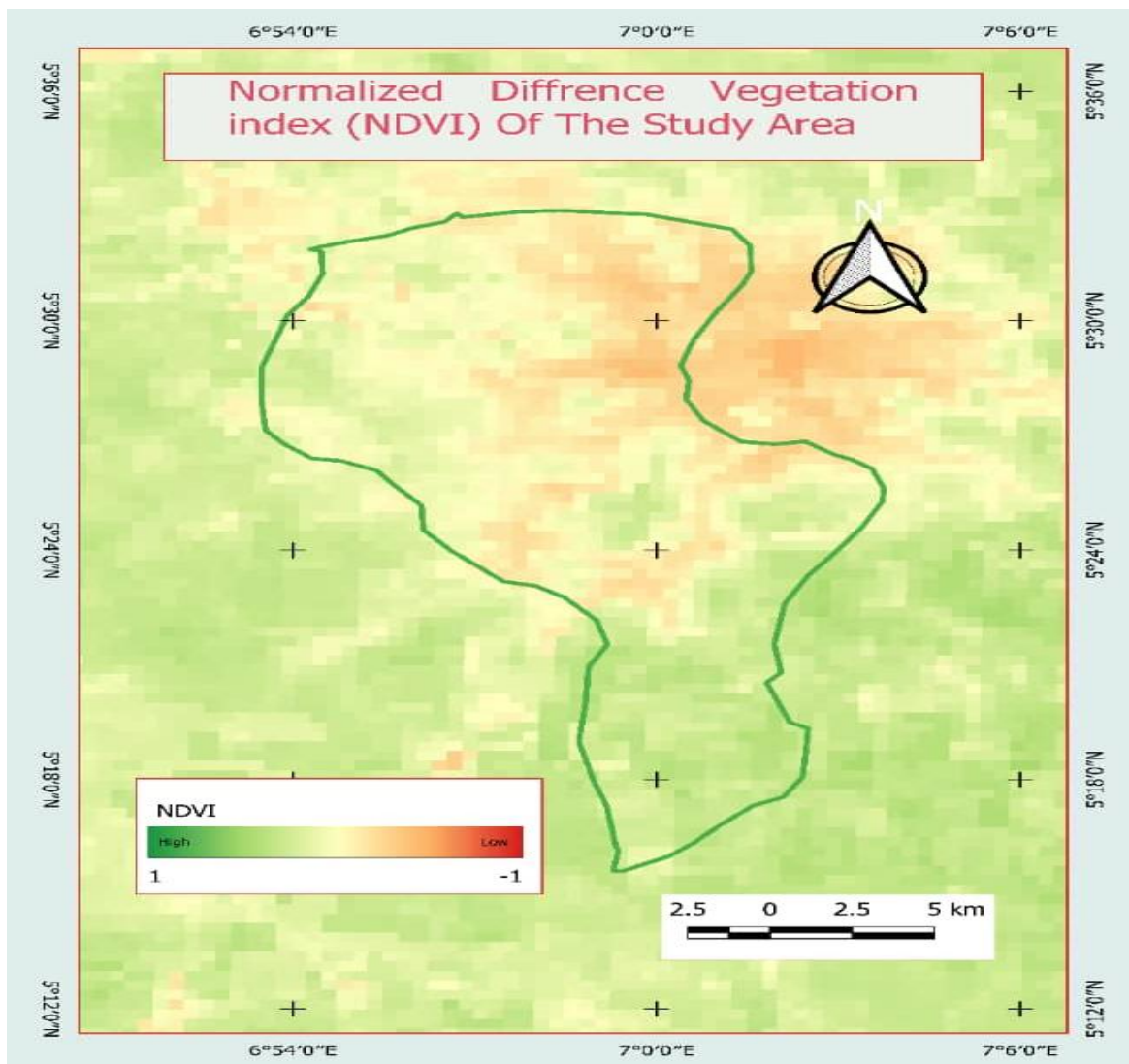
Fig. 2. NDVI of the area
