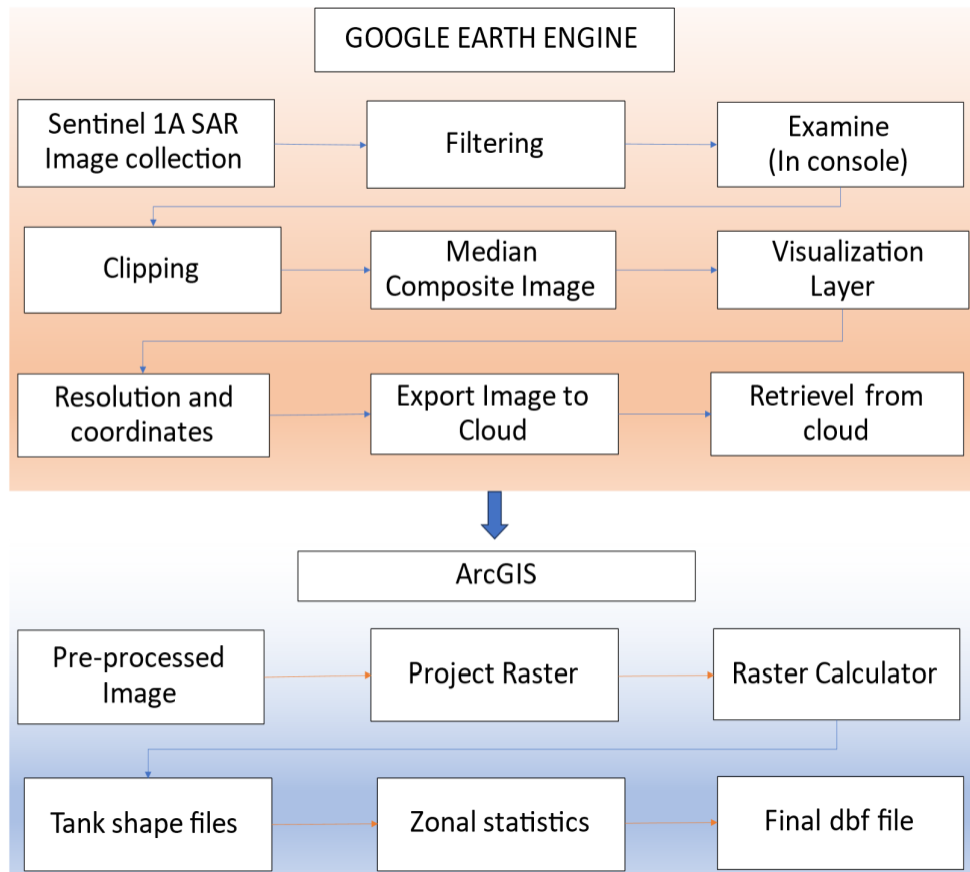
Fig. 3. Methodology adopted for mapping of water spread area
