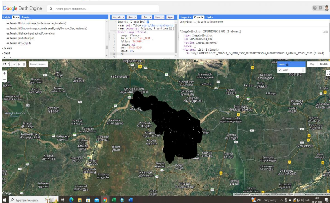
Fig. 2. Overview of preprocessed Sentinel 1A image acquisition for the study area
