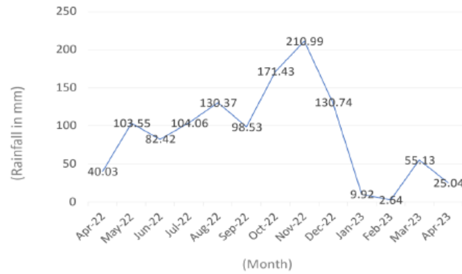
Fig. 4. Rainfall pattern for Cuddalore district from April-2022 to April-2023
