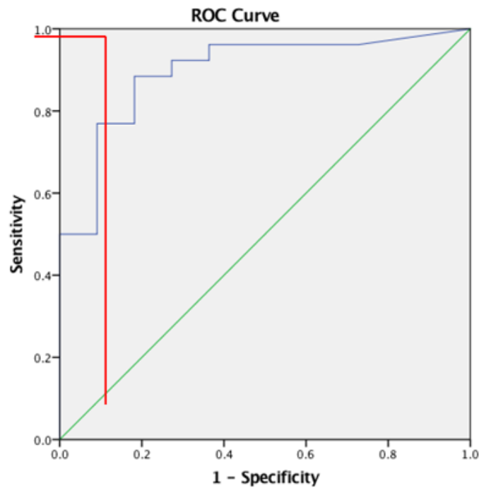
Fig. 4. PCT ROC curve in sepsis patients
