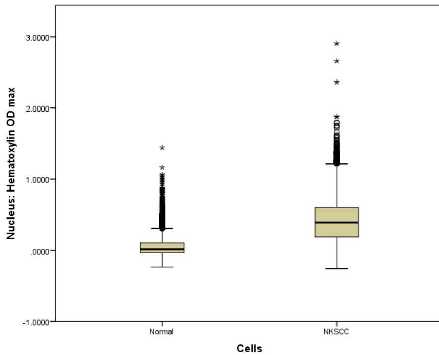
Fig. 5. Boxplot of maximum nucleus hematoxylin OD for normal and non-keratinizing squamous carcinoma cells. The box-plot above shows that most malignant cells have higher maximum (max) nuclei hematoxylin OD than the normal cells ( p < 0.001 )
