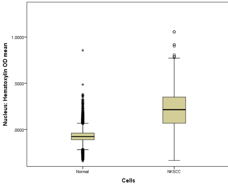
Fig. 3. Boxplot of nucleus hematoxylin OD mean of normal and non-keratinizing squamous carcinoma cells. The box-plot above shows that most malignant cells have higher nuclei hematoxylin OD mean than the normal cells ( p<0.001 )
