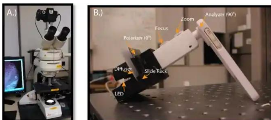
Fig. 4. Pictorial demonstration of malaria diagnosis using a mobile phone polarized microscope. (A) Leica Direct Metal Laser Melting (DMLM) polarized white light microscope used as reference for comparison. And (B) a microscope lens combination implemented into a 3D-printed fitting to allow similar function to a traditional polarized microscope. The Mobile-optical-polarization-imaging device (MOPID) system configured in transmission mode with a magnification designed for 40x when using a mobile phone camera. An iPhone 5s is used with polarizer sheets added and a 3D-printed fitting to hold the light source, diffuser, sample slide and microscope attachment [54]
