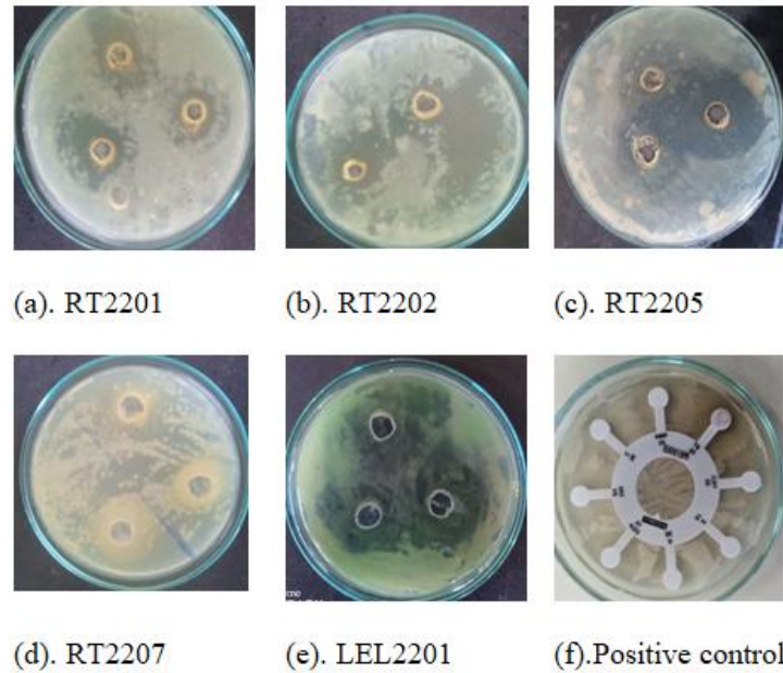
Plate 4. Images of zones of inhibition of selected Actinomycetes isolates (RT2201 (8.5 mm), RT2202 (4.0 mm), RT2205 (7 mm), RT2207 (1.5 mm) and LEL2201 (25 mm) against S. aureus . The isolates were grown on MHA for 24 hours at 28°C. The positive control is a disk with various drug concentrations. TE-tetracycline, K-kanamycin, COT-cotrimoxazole, AMP -ampicillin, S-streptomycin, Sx-sulphamethoxazole, GEN-gentamicin, and C-chloramphenicol. The S. aureus is sensitive to all of them
